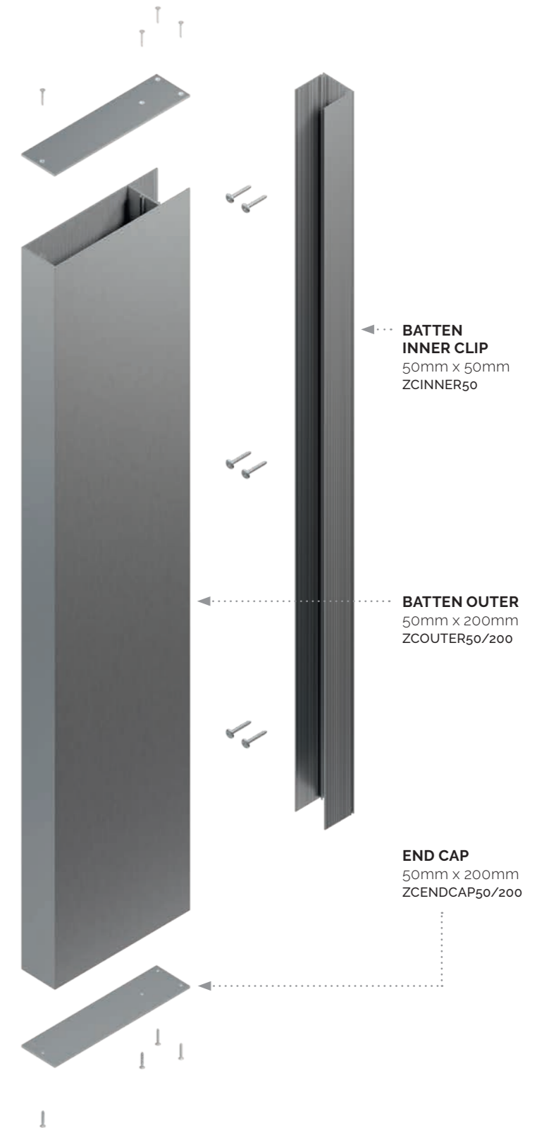
*50mm x 200mm Batten System displayed for illustrative purposes - batten outer illustrated is indicative option only.
